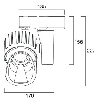
Beacon Shelf DALI - front view
