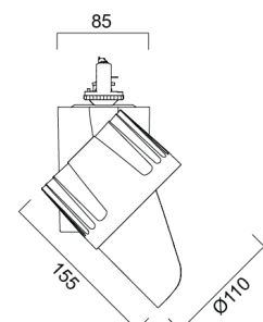
Beacon Shelf DALI- side view
